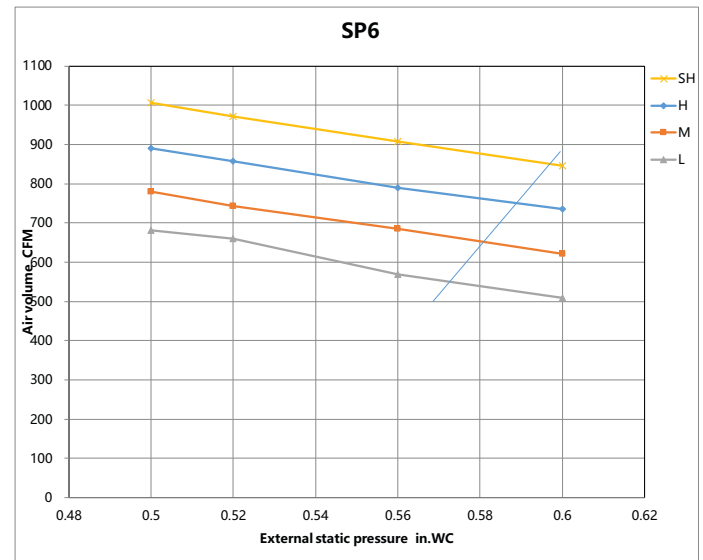
Fig. 28 – High Static Pressure Curves - 24k
