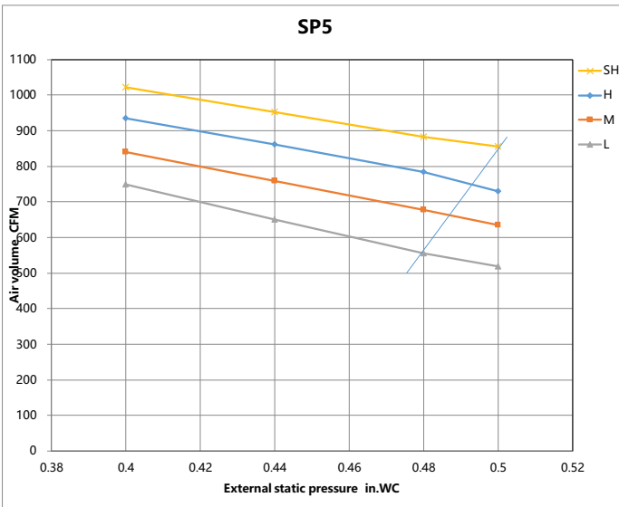
Fig. 28 – High Static Pressure Curves - 24k
