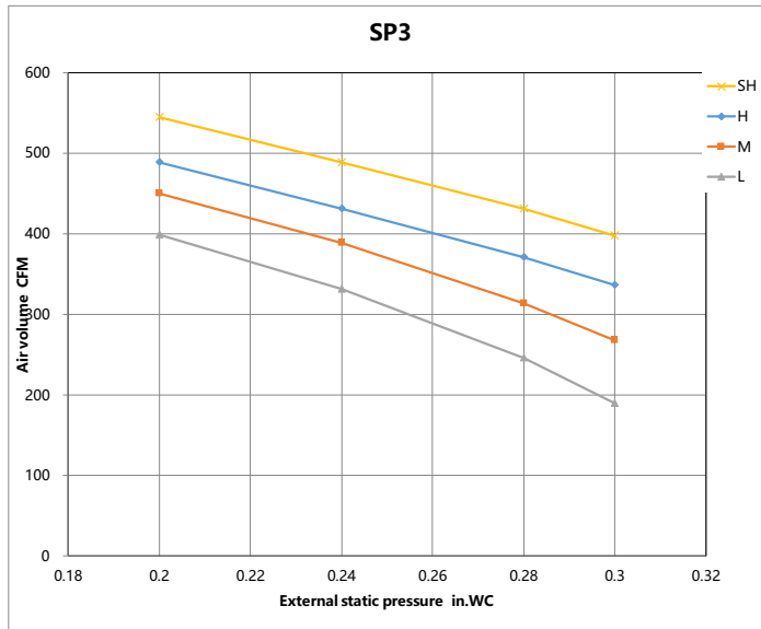
Fig. 18 – Low Static Pressure Curves – 12k
