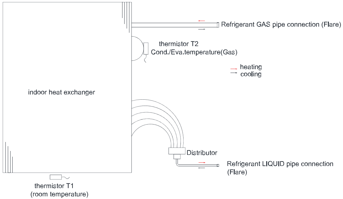
Fig. 37 – Refrigerant System Diagram
