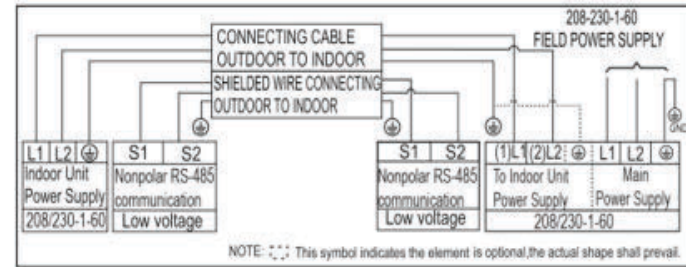
Fig. 11 – 36K Connection Label
