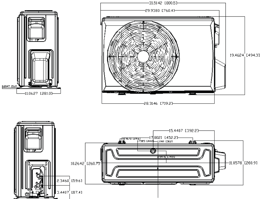
Fig. 2 — Sizes 9K/12K (115V) and 9K/12K (208/230V) Heat Pump
