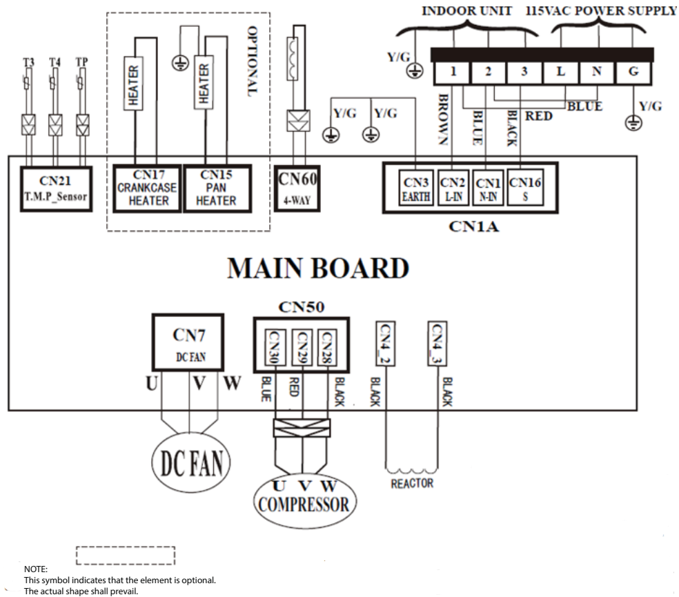
Fig. 8 — Wiring Diagram Heat Pump Size 9K - 12K (115V)
