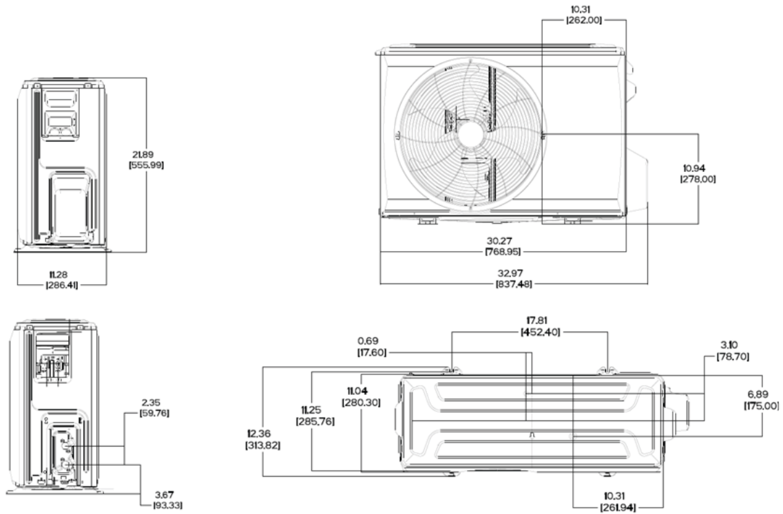
Fig. 3 — Size 18K Heat Pump
