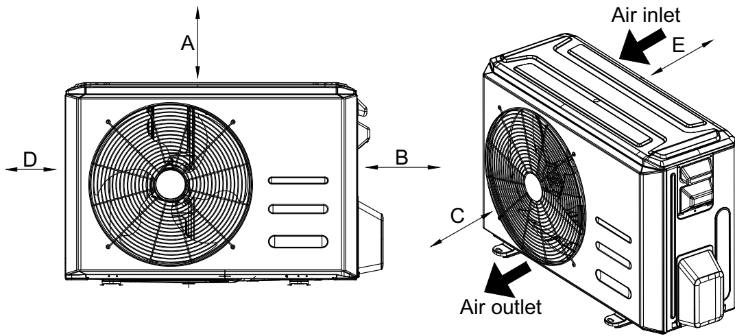
Fig. 5 — Clearances
