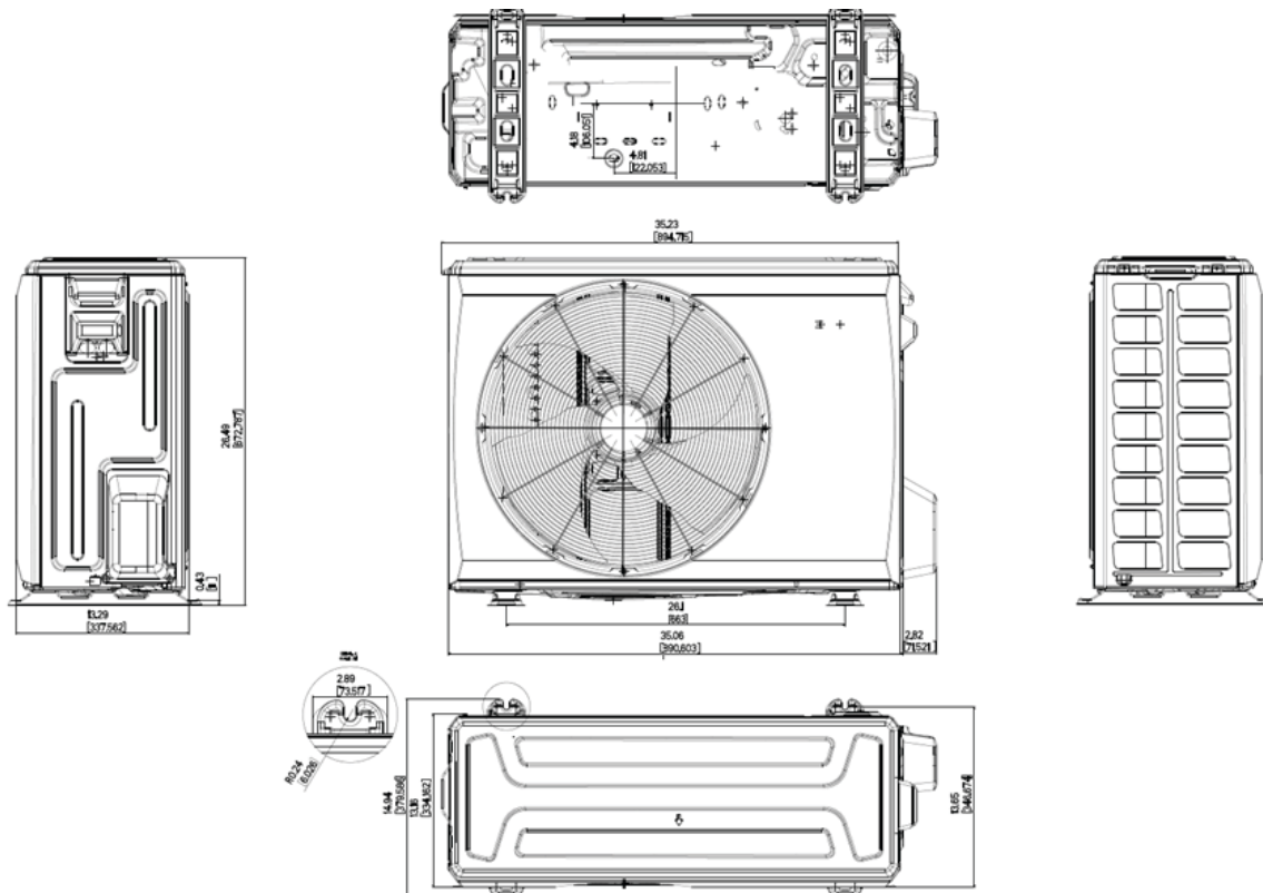
Fig. 4 — Size 24K Heat Pump
